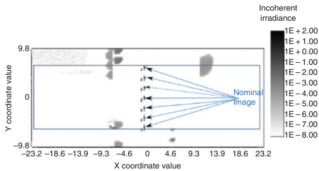
Figure 16: Tilt of 1^\circ in the y-direction of Lens 1.
