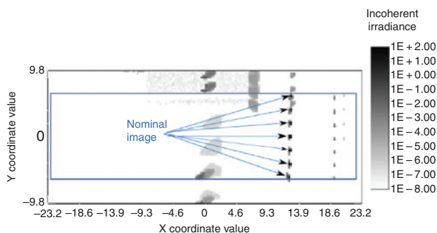
Figure 19: Combined M1 + M2 tilted by 1^\circ and L1 by -1^\circ in the y-direction.
