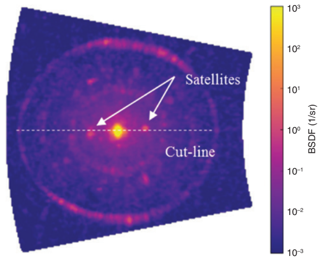
Figure 7: 3D BSDF map of the grating at the -1 st order peak (range \varphi_s = -13^\circ – 13^\circ and \theta_s = -43.4^\circ – 25.4^\circ ) feature showing the angle of the satellites.
