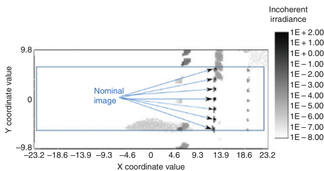
Figure 17: Tilt of 1^\circ in the y-direction of Mirror 1 & 2.
