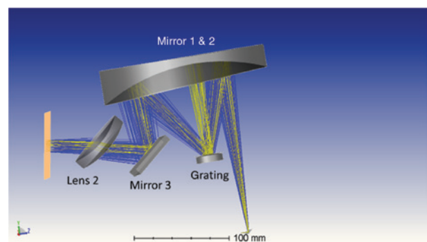
Figure 21: Nominal ray path (blue) and parasitic path (yellow) for the optimized system.
