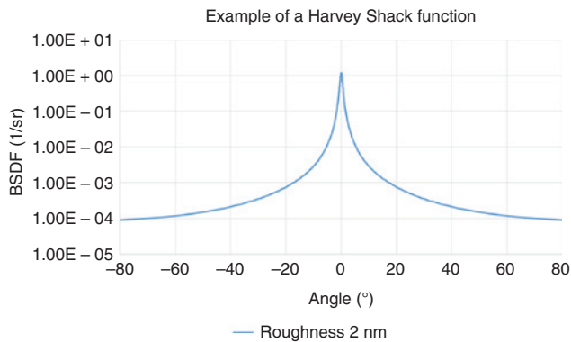
Figure 1: Example of a BSDF approximated by a Harvey-Shack function for a mirror with 2 nm roughness at 532 nm wavelength.
