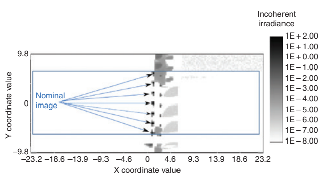
Figure 18: Tilt of 1^\circ in the y-direction of the grating.
